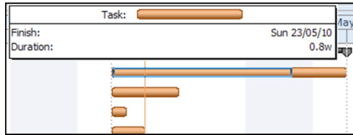
Figure 6-16: Adjusting Duration
