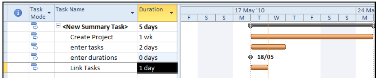
Figure 4-12: A Milestone
