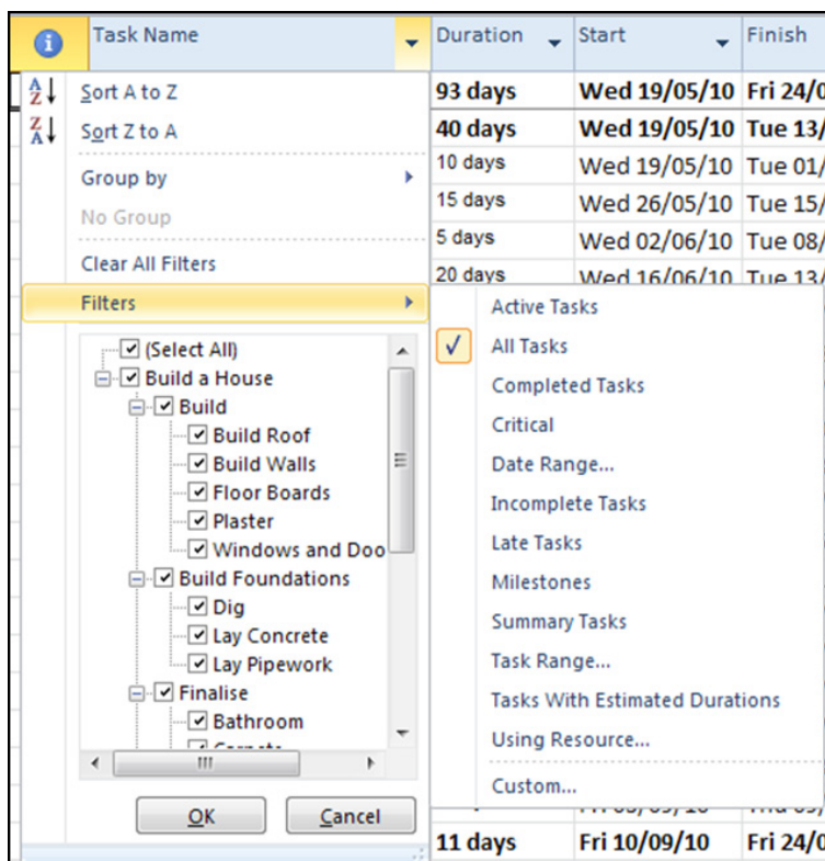
Figure 6-19: Filter Options
