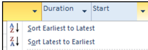
Figure 6-21: Sort Options
